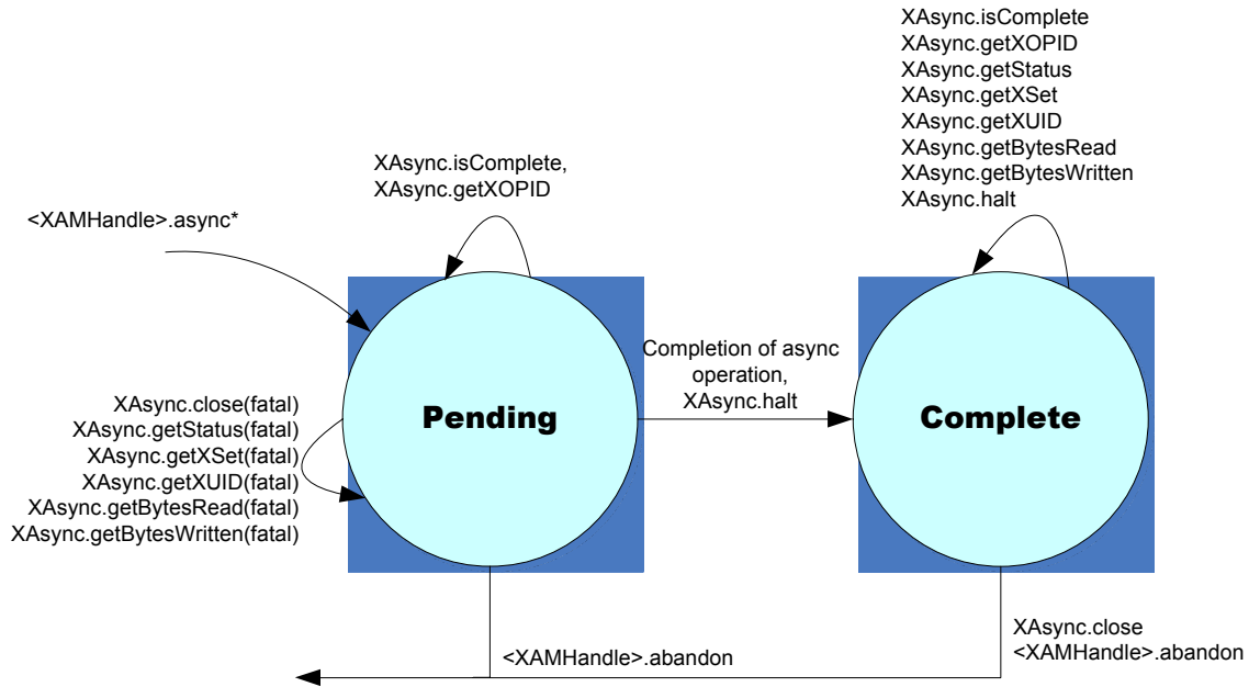
Figure 20 – XAsync Instance FSM
