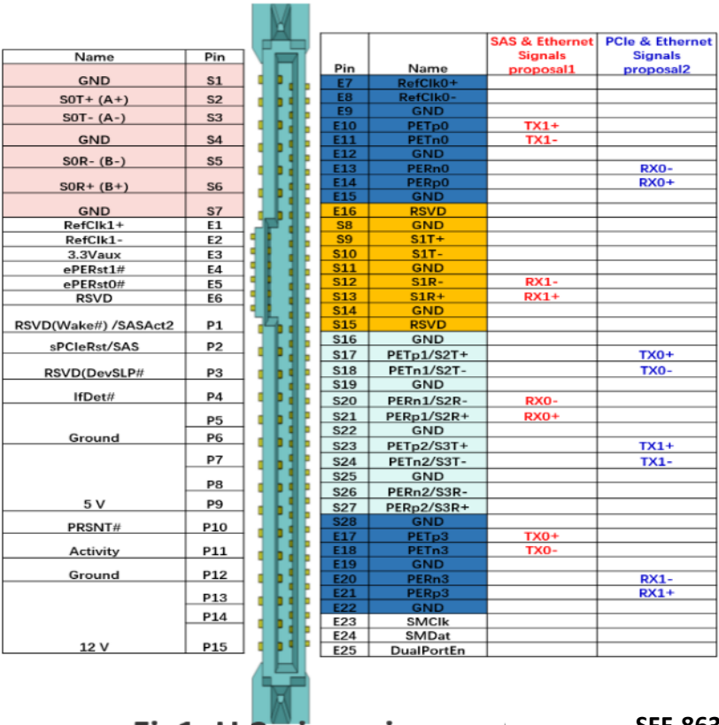
SFF-8639 connector
