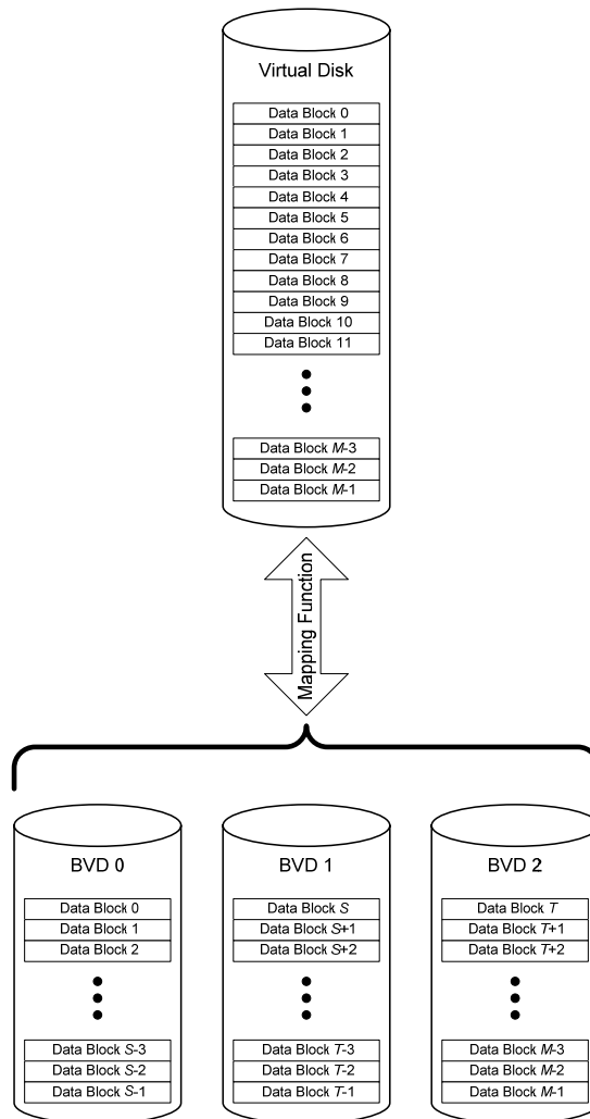
Figure 24: Concatenated Secondary RAID Level (SRL=02)
