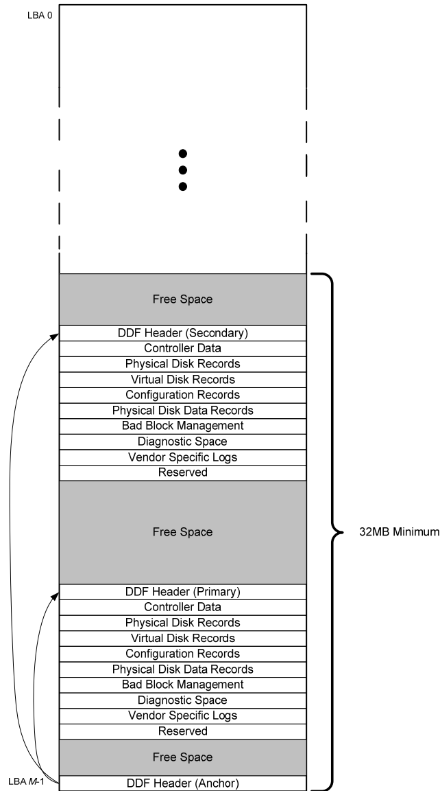
Figure 26: DDF Structure
