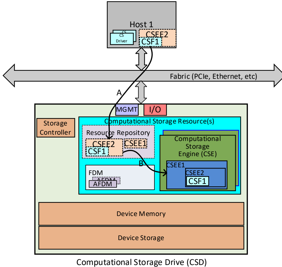
Figure B.2.7 – CSx Configuration process
