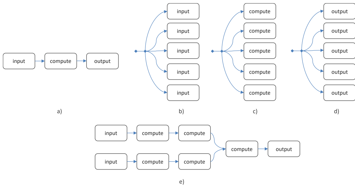
Figure 12: Batch Requests
