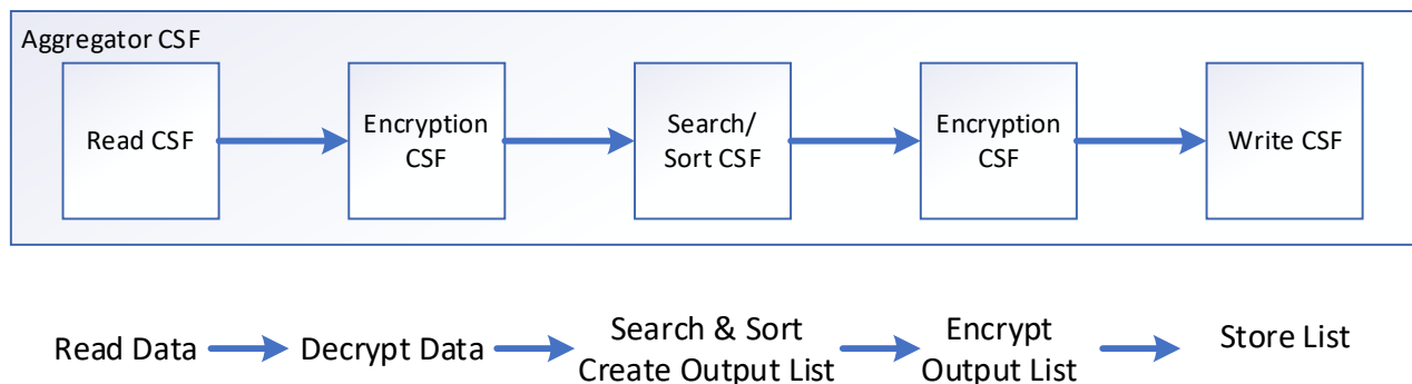
Figure 4.5 – Fixed Sequence Aggregator
