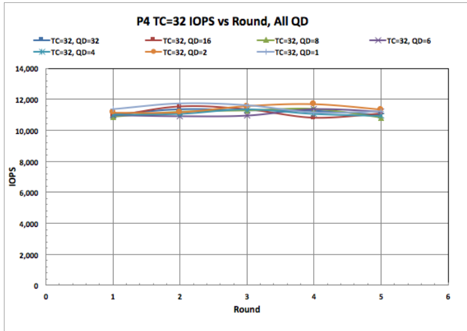
Plot 13-7 - DV IOPS Plot, TC=Tracking
