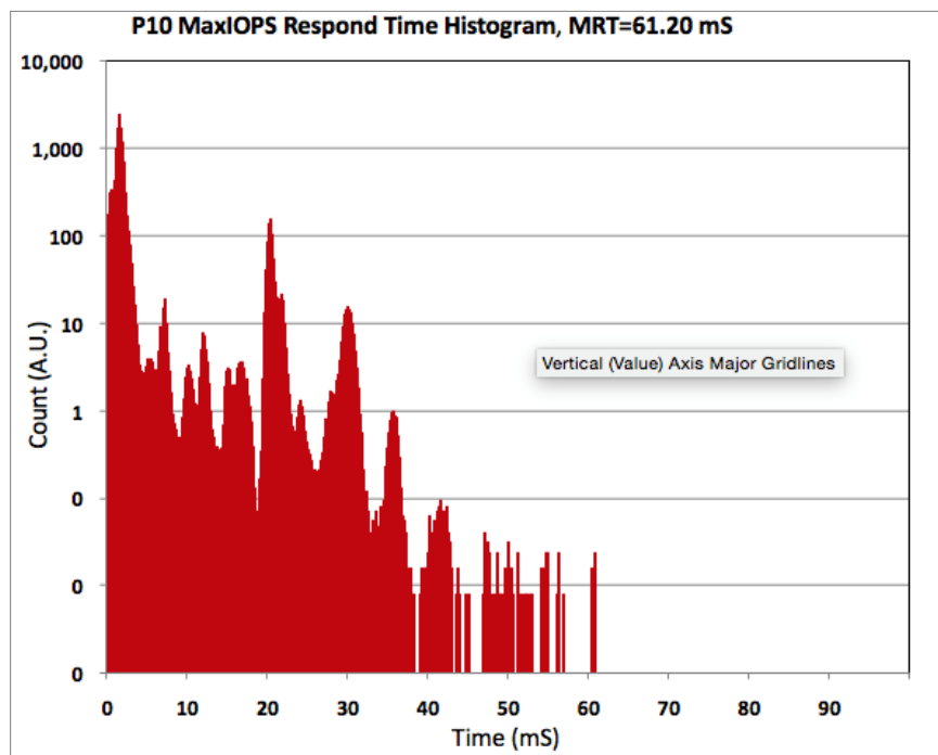
Plot 14-11 - Max IOPS Histogram
