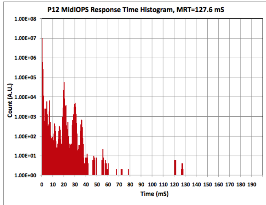
Plot 13-15 - MidIOPS Histogram
