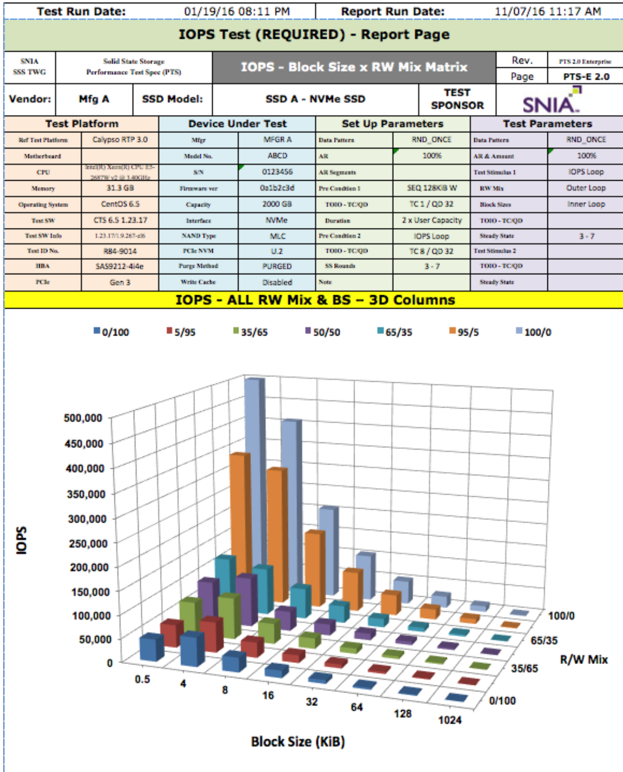
Plot A.8 – IOPS -All RW Mix & BS - 3D Columns
