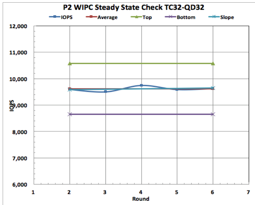
Plot 14-3 - Pre-Conditioning Steady State Plot
