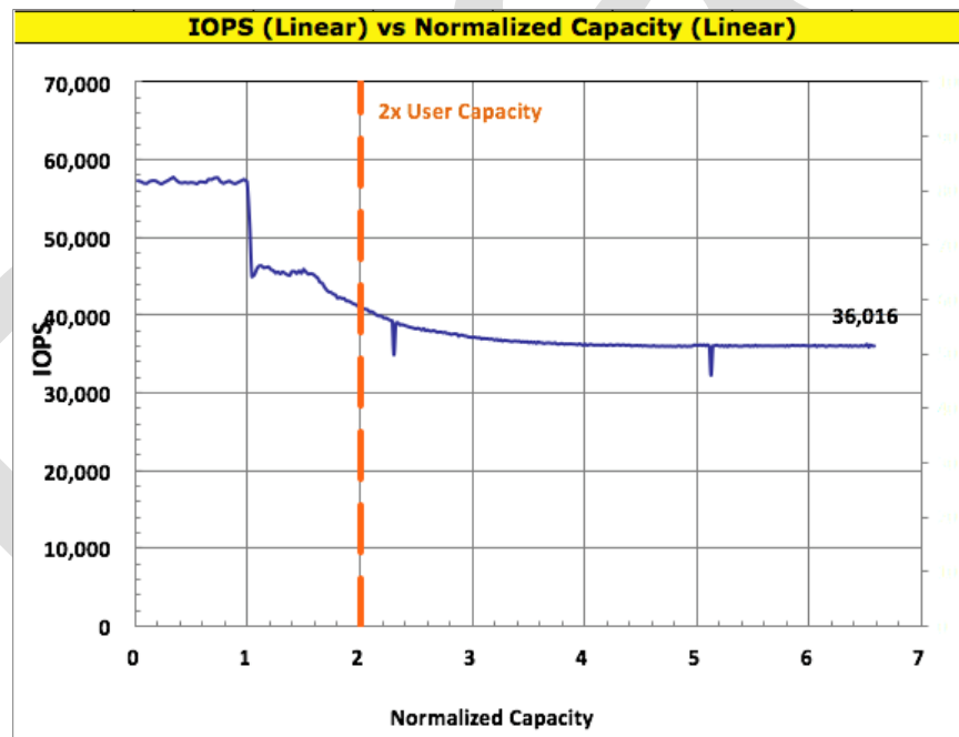
Plot 10-3 - WSAT IOPS v Total Drive Writes/Fills
