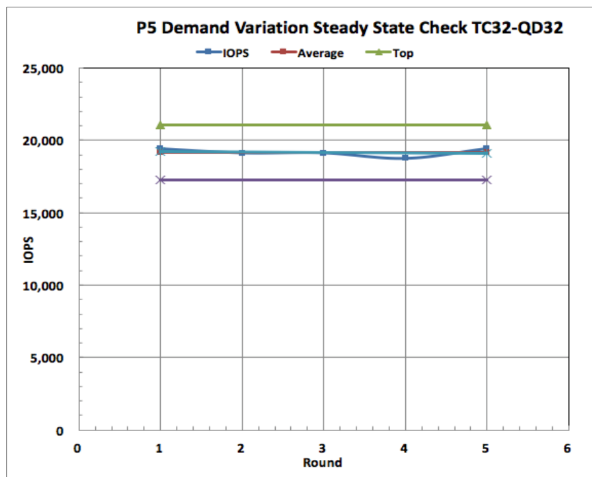
Plot 14-6 - DV Steady State Plot, Tracking Variable
