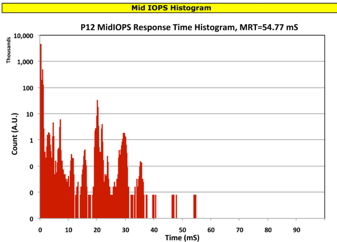
Plot 14-13 - Mid IOPS Histogram
