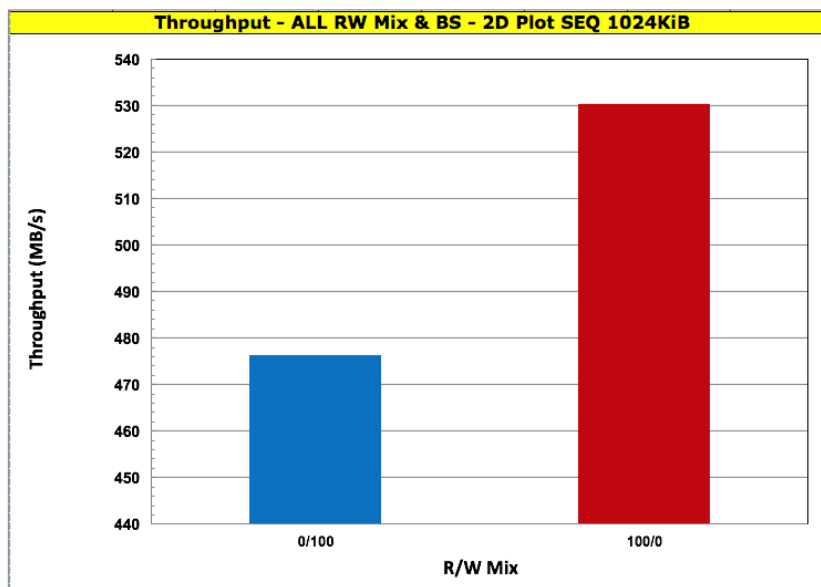
Plot 8-6 - TP Measurement Plot – 2D SEQ 1024KiB
