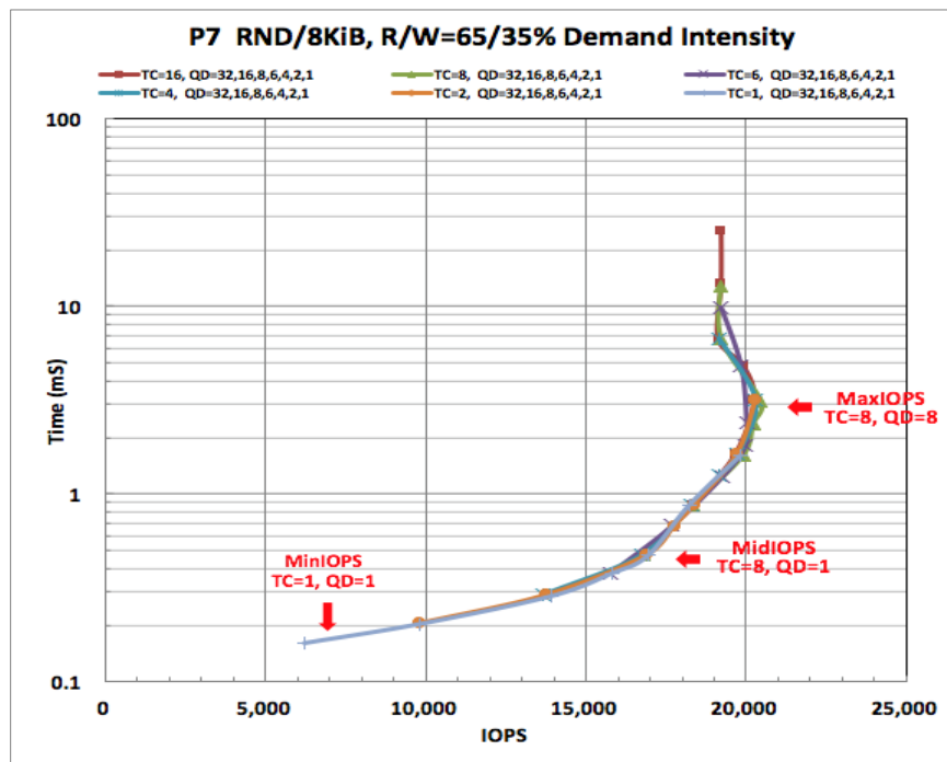
Plot 14-8 - Demand Intensity Plot
