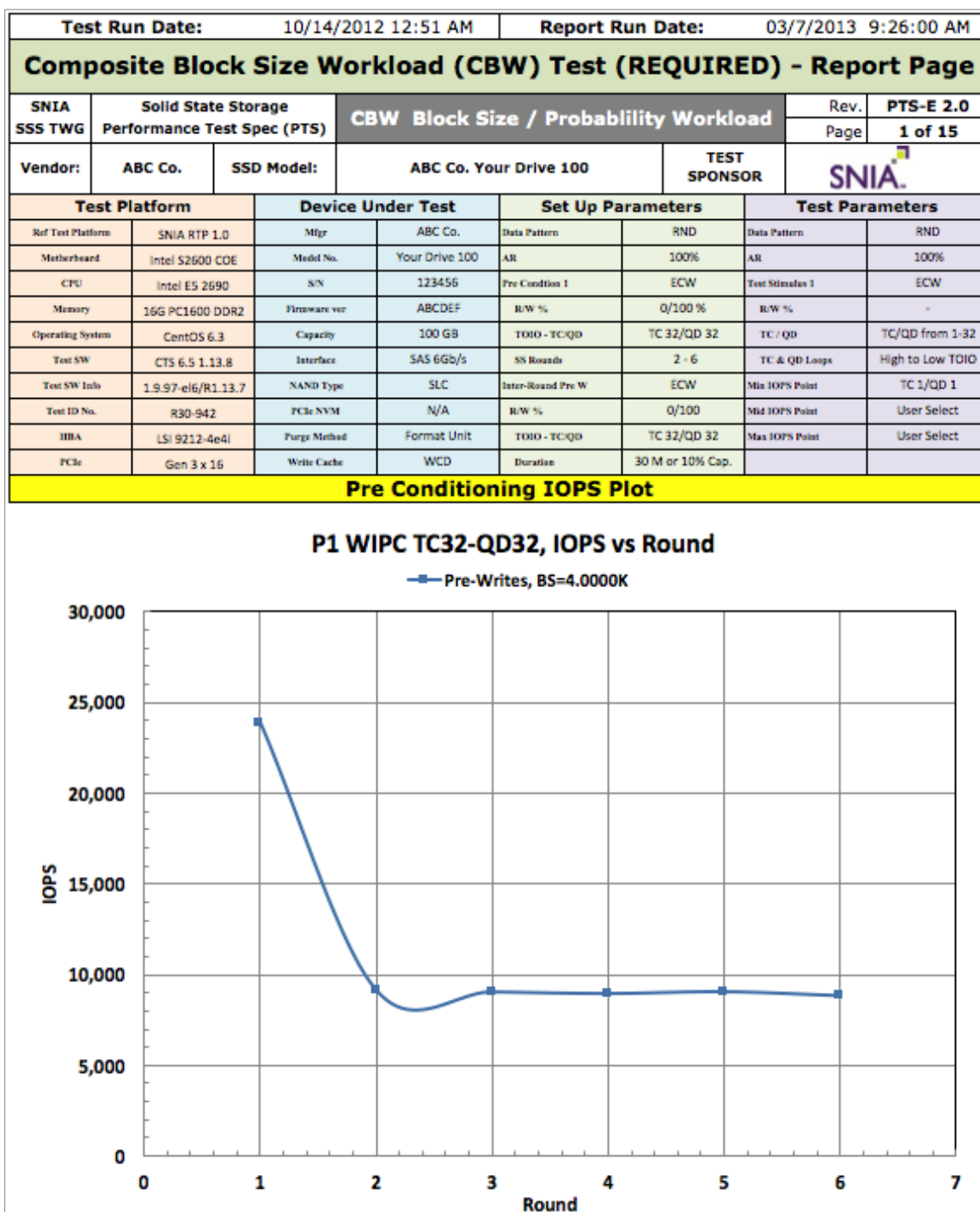
Plot 13-4 – Pre-Conditioning IOPS Plot
