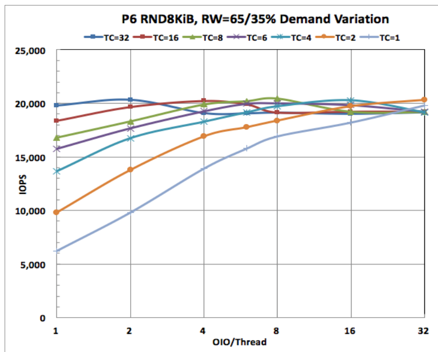
Plot 14-7 - Demand Variation Plot
