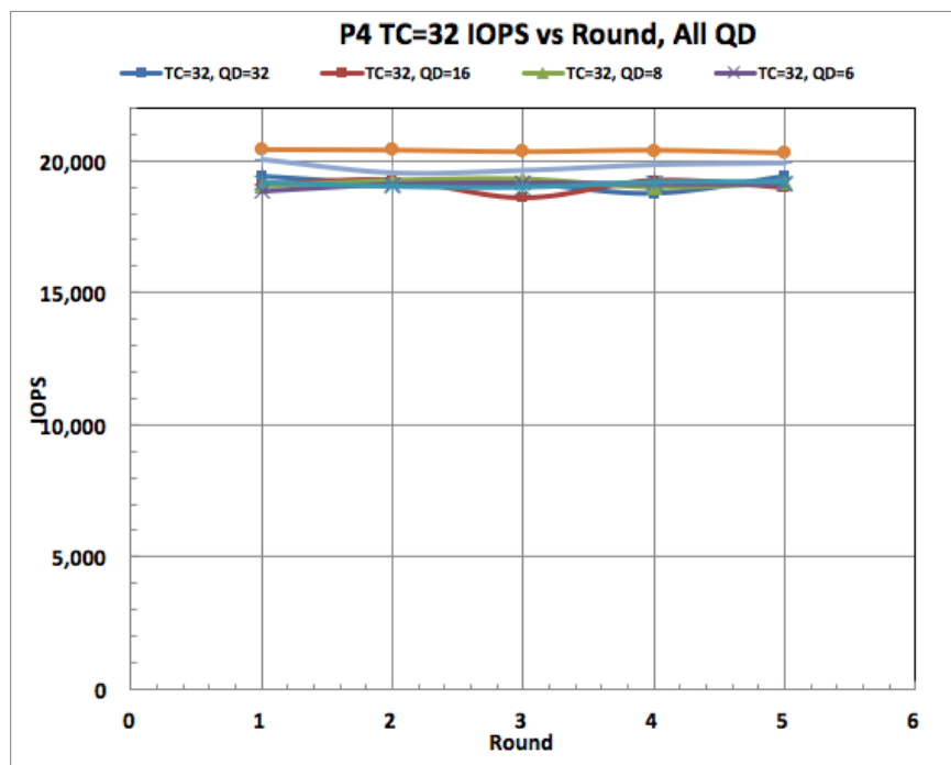
Plot 14-5 - DV IOPS Plot, TC=Tracking
