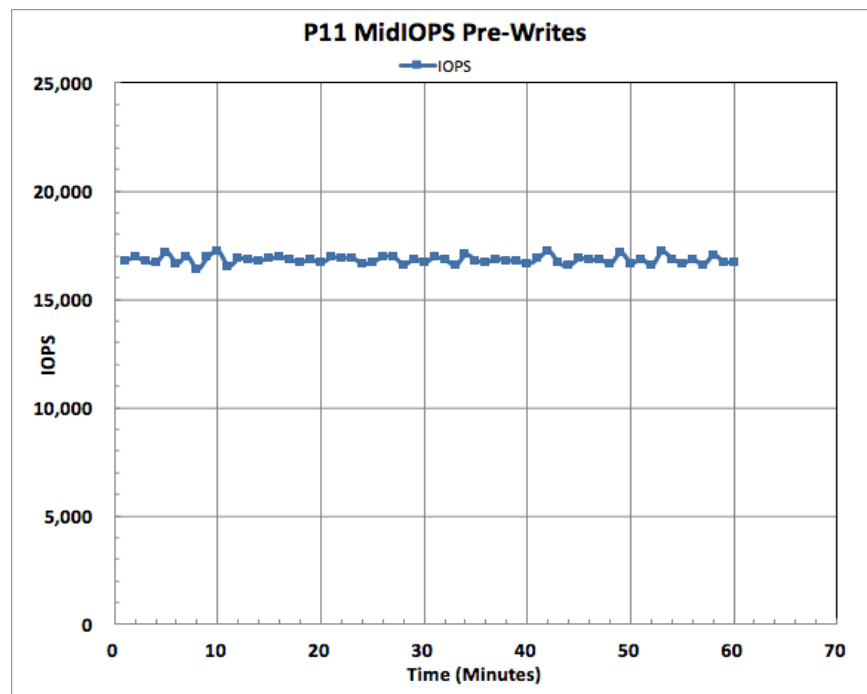
Plot 14-12 - Mid IOPS Pre Writes
