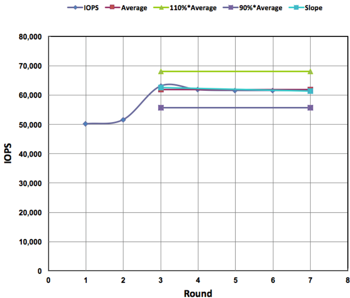
Plot A.3 – IOPS Steady State Measurement Window - RND/4KiB
