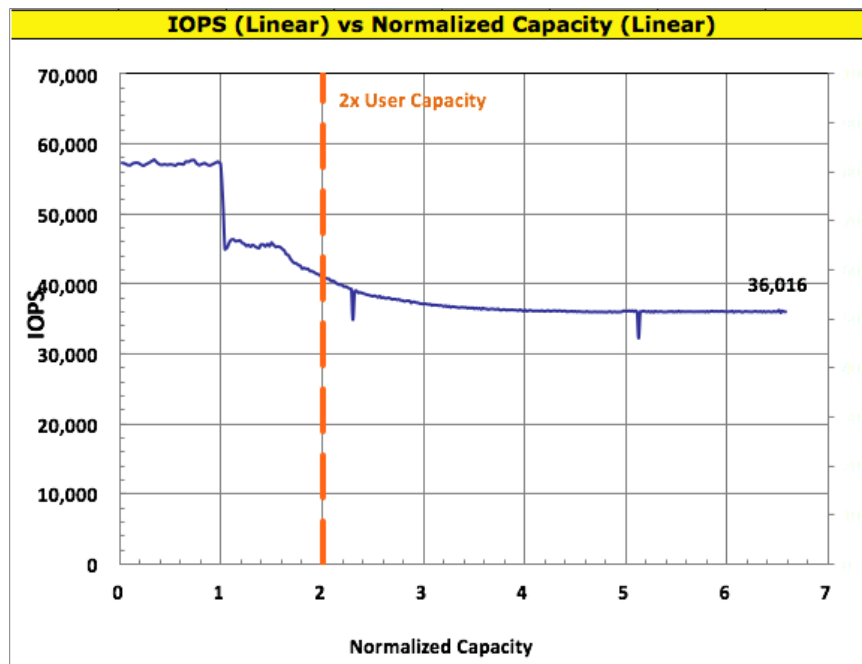
Plot 10-3 - WSAT IOPS v Total Drive Writes/Fills
