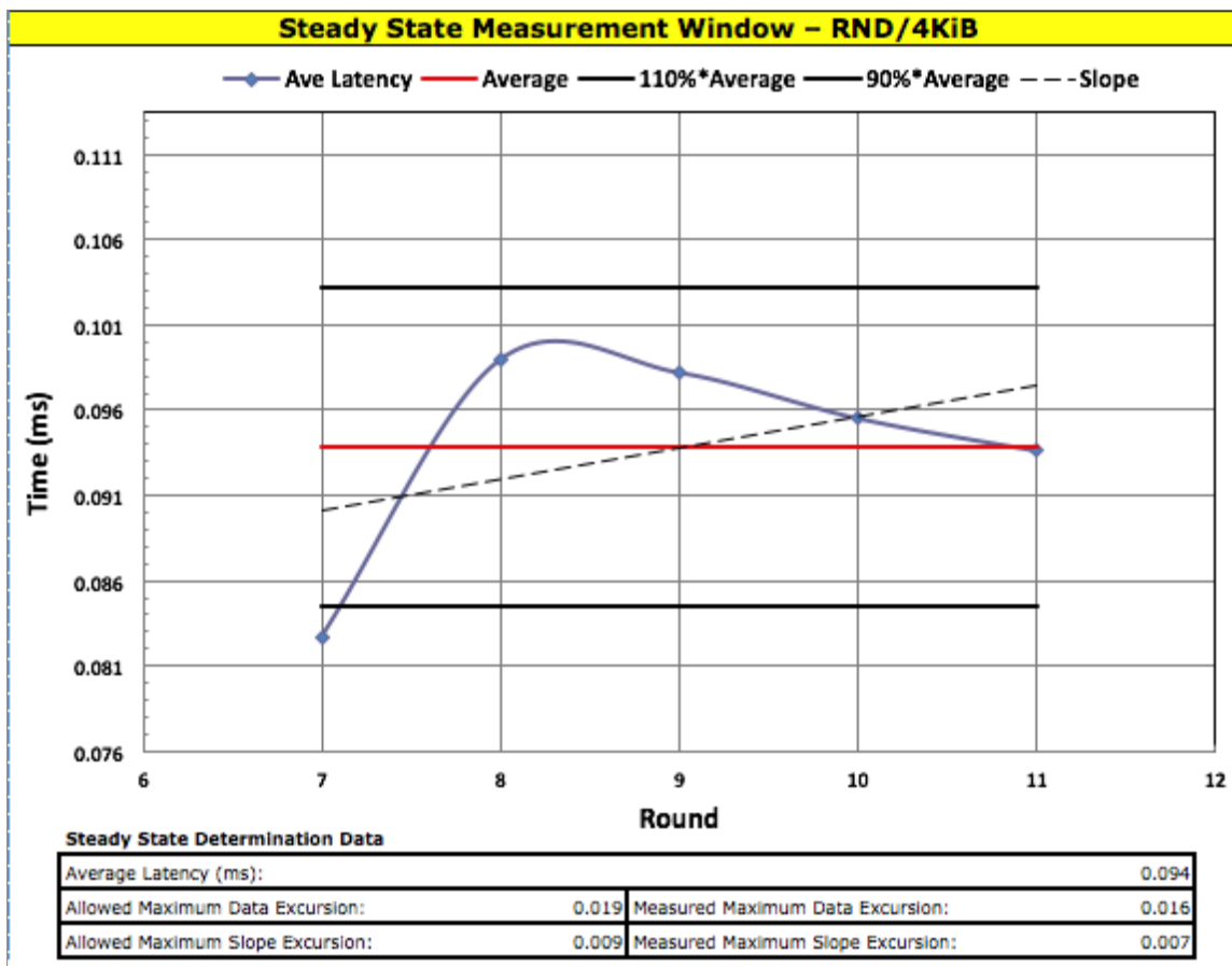
Plot 9-2 - LAT SS Measurement Window
