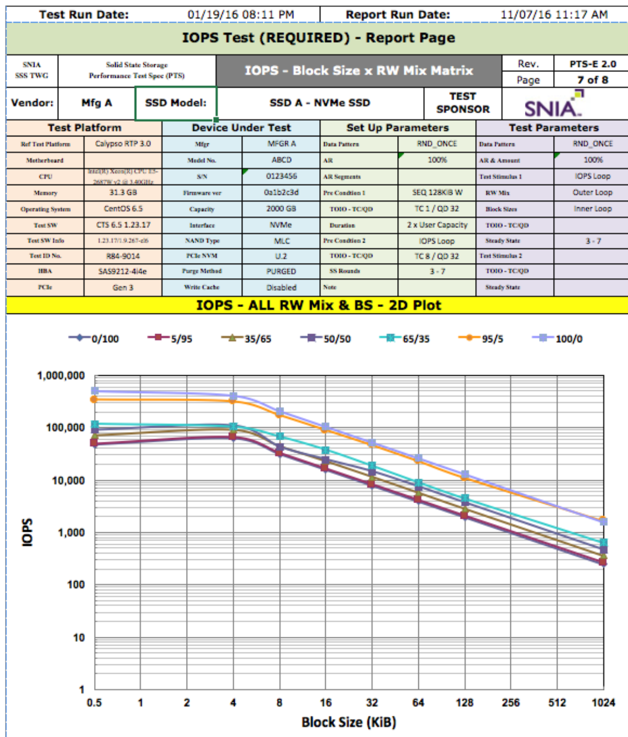
Plot A.7 – IOPS – Table BS / RW Mixes
