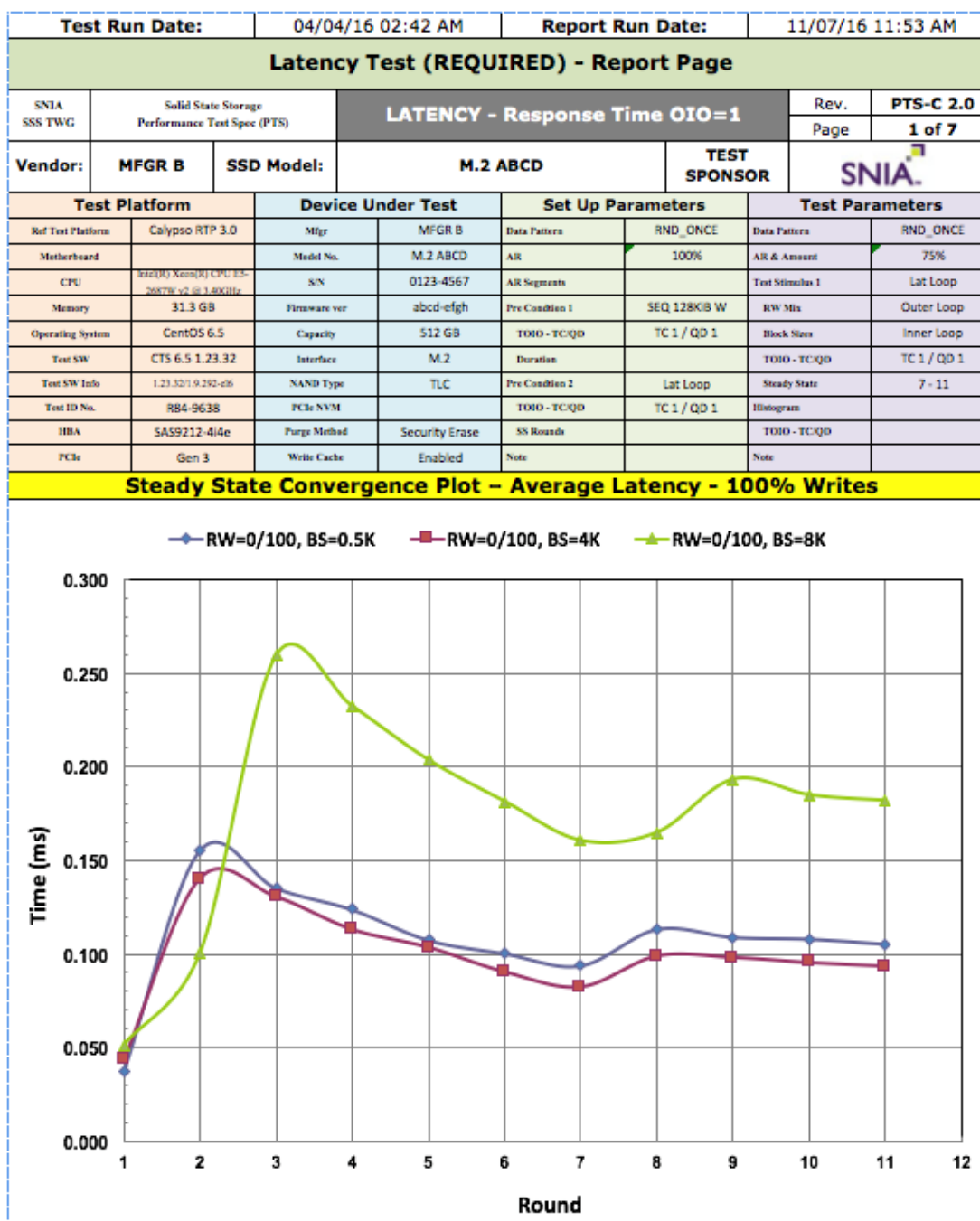
Plot 9-1 - LAT SS Convergence Report
