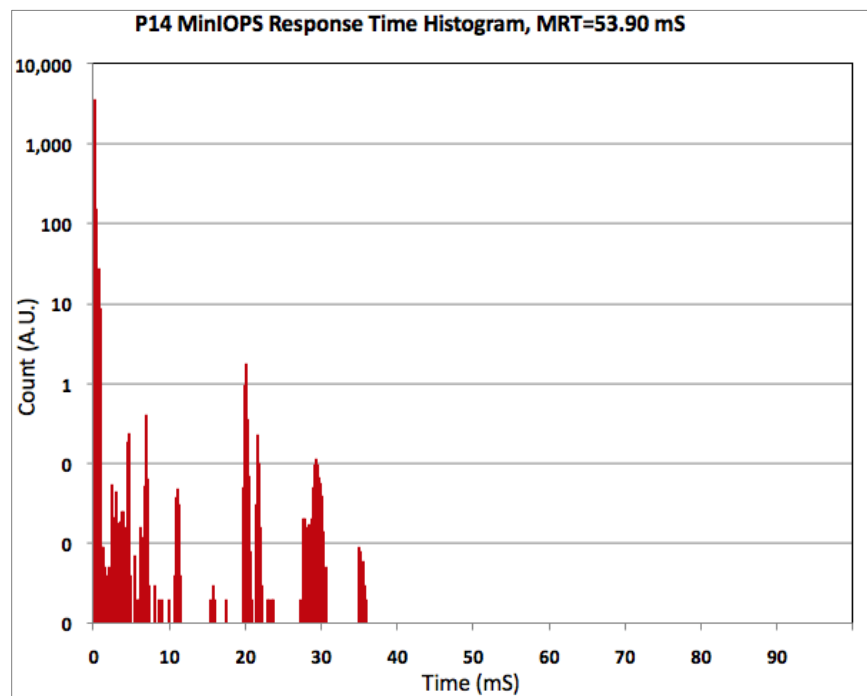
Plot 14-15 - Min IOPS Histogram
