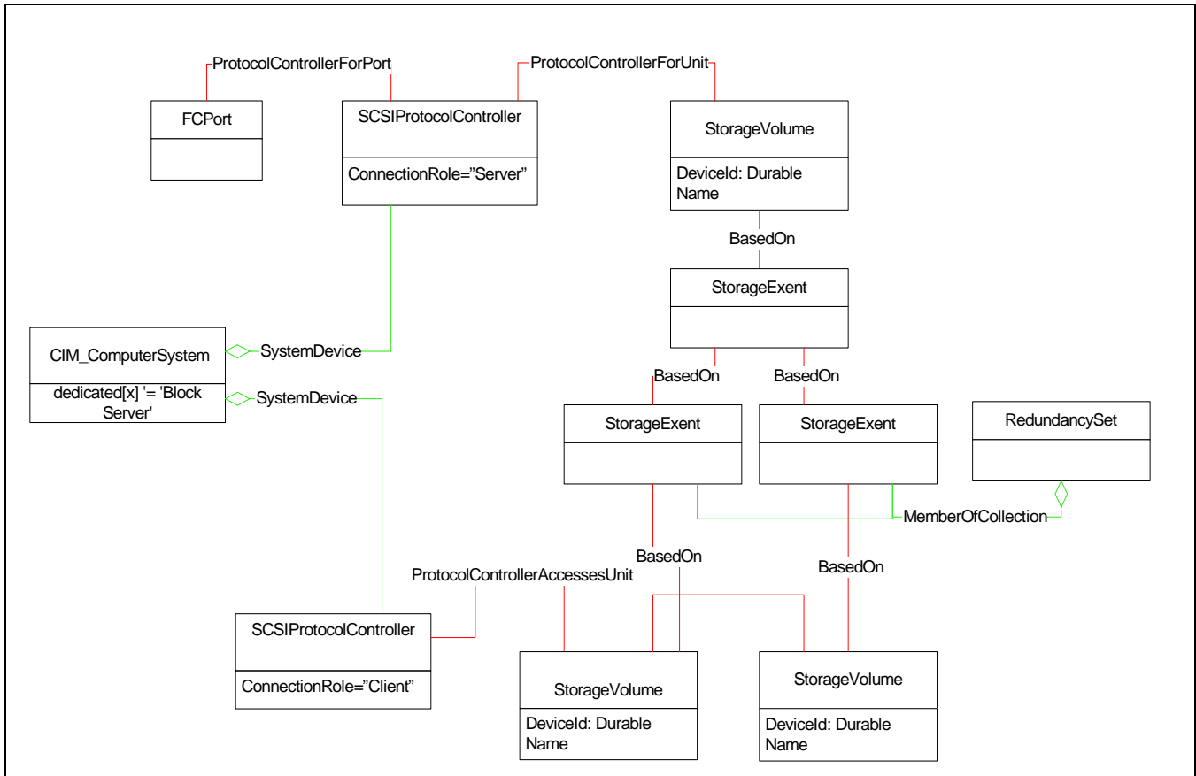
Figure 73 - Array Instance
