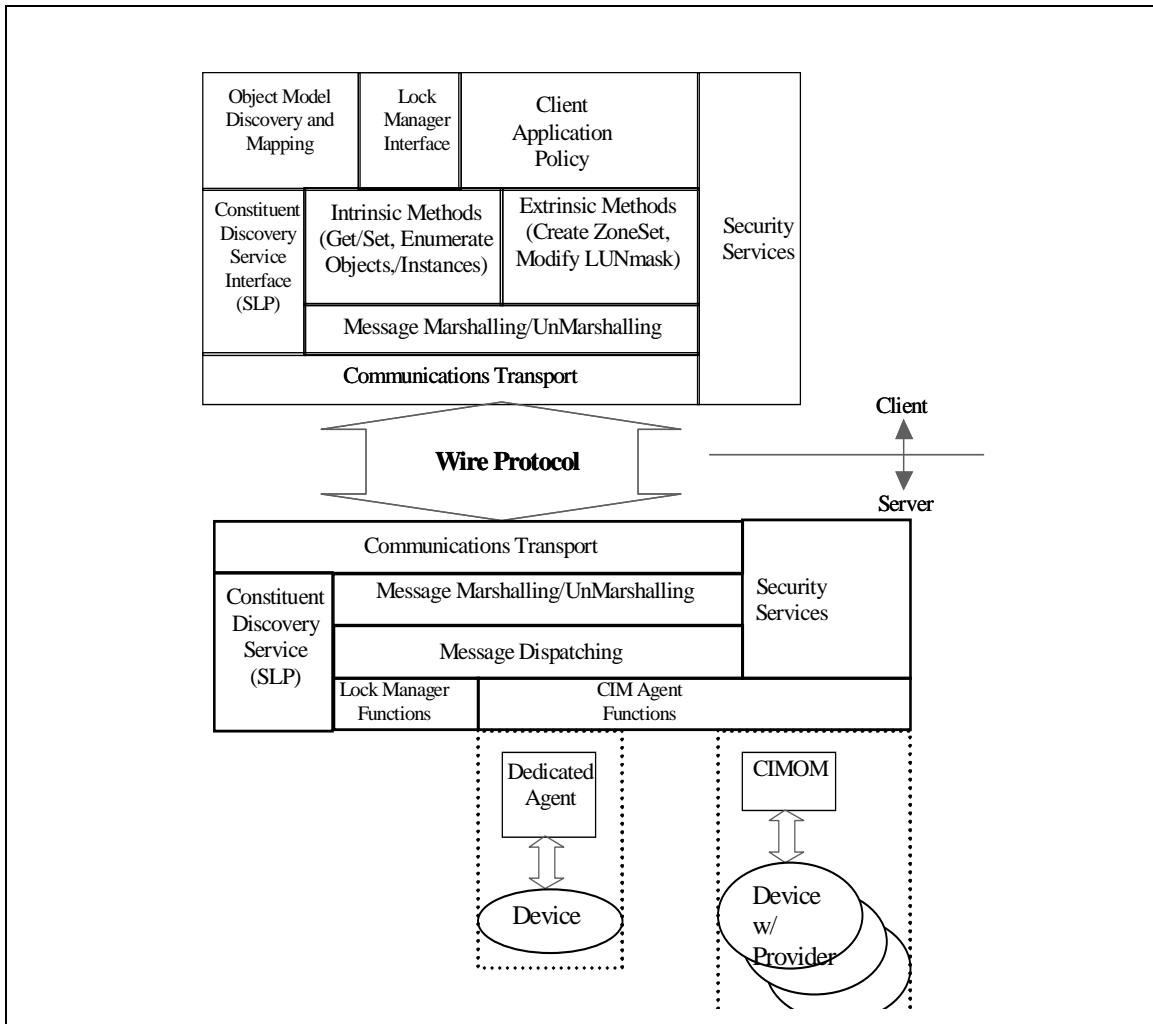
Figure 8 - Operational environment
