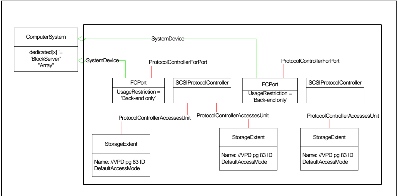
Figure B.14 - Translation Engine Back-end Ports Instance
