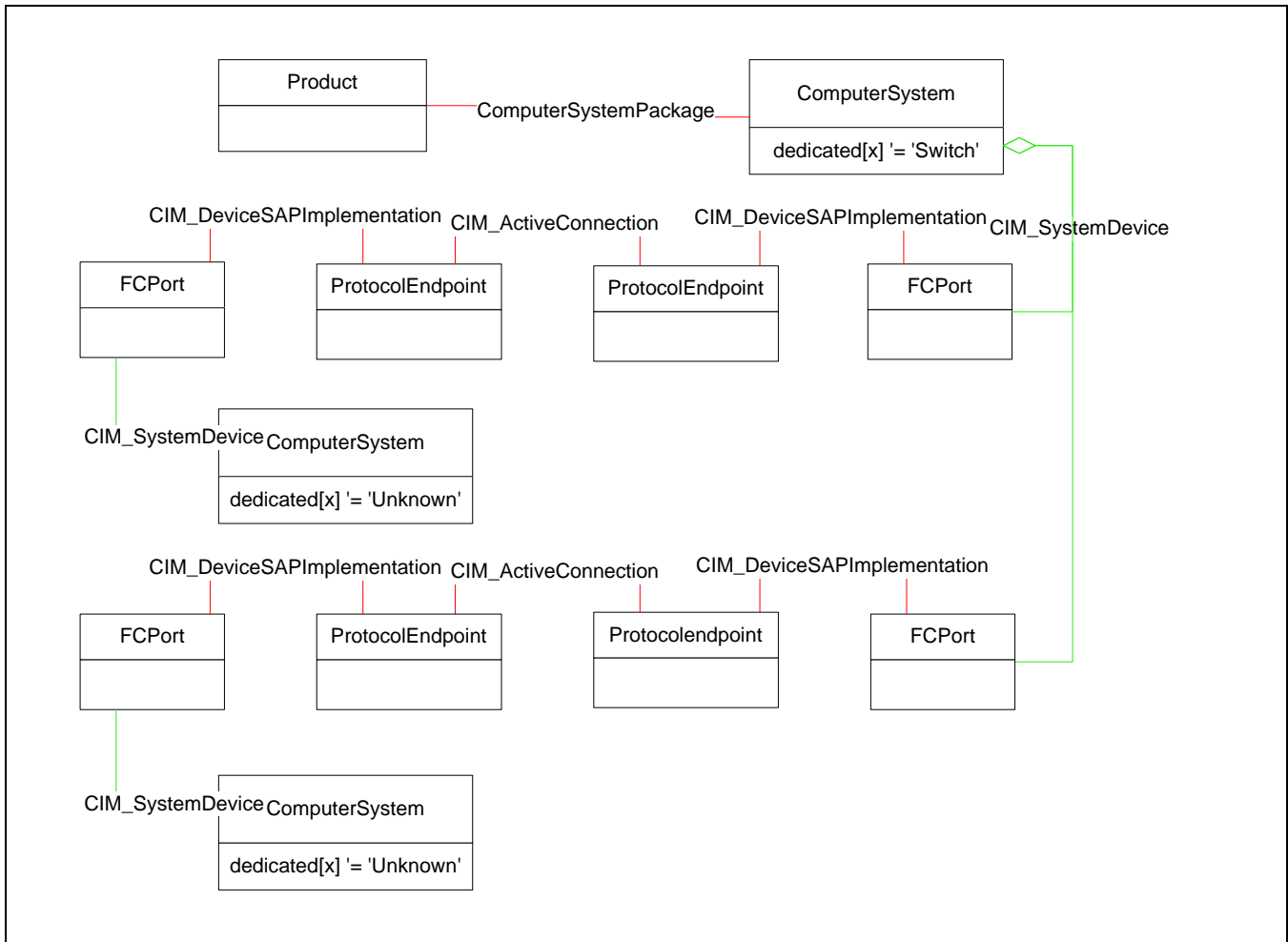
Figure 72 - Switch Model
