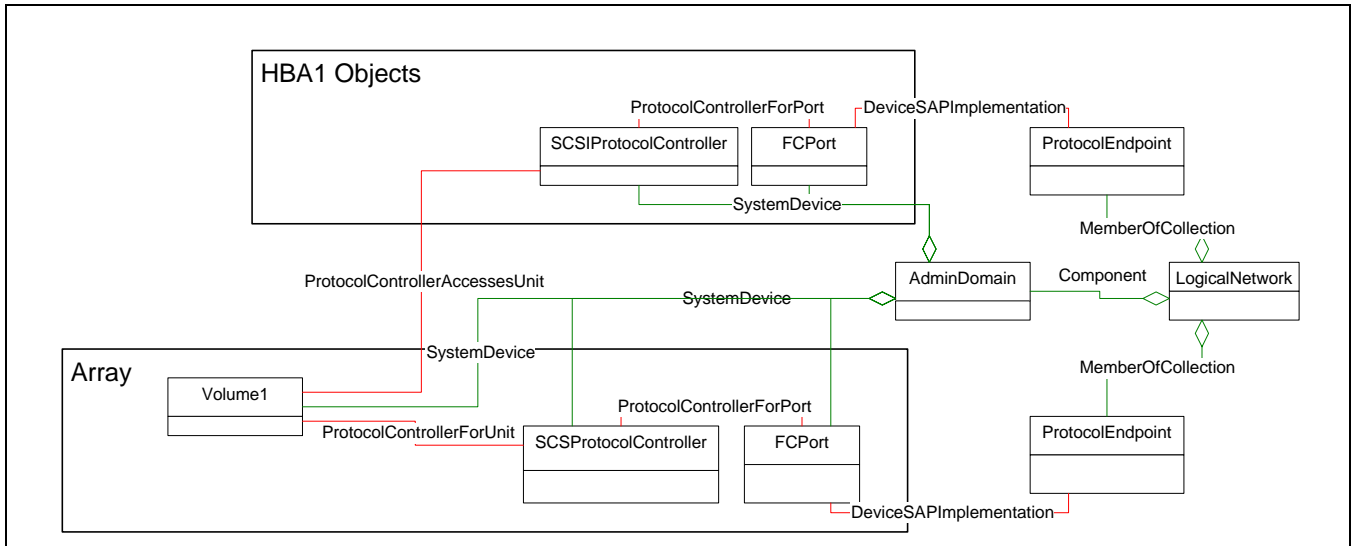
Figure B.18 - Host Discovered Resources Instance Diagram 2
