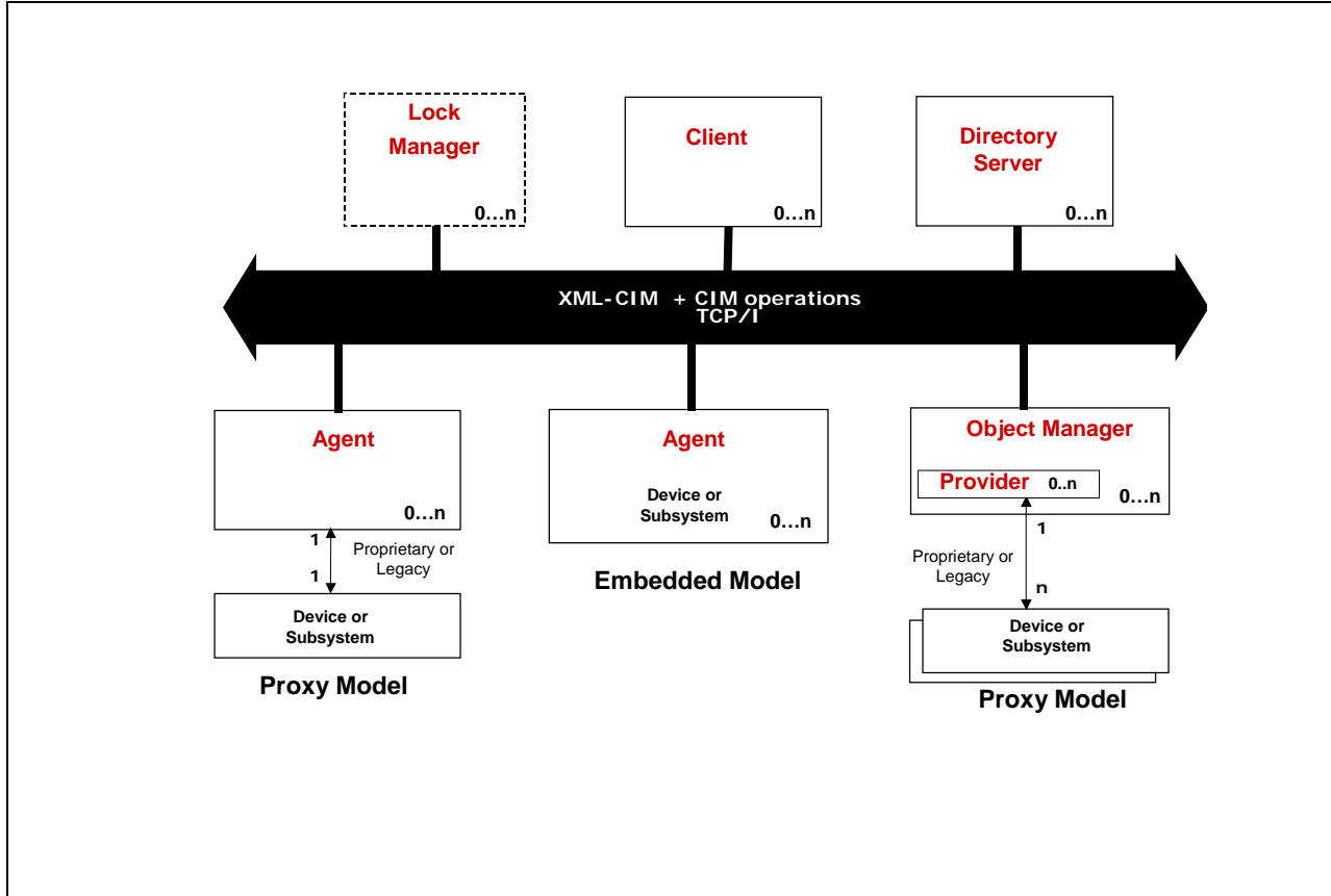
Figure 10 - Reference Mode
