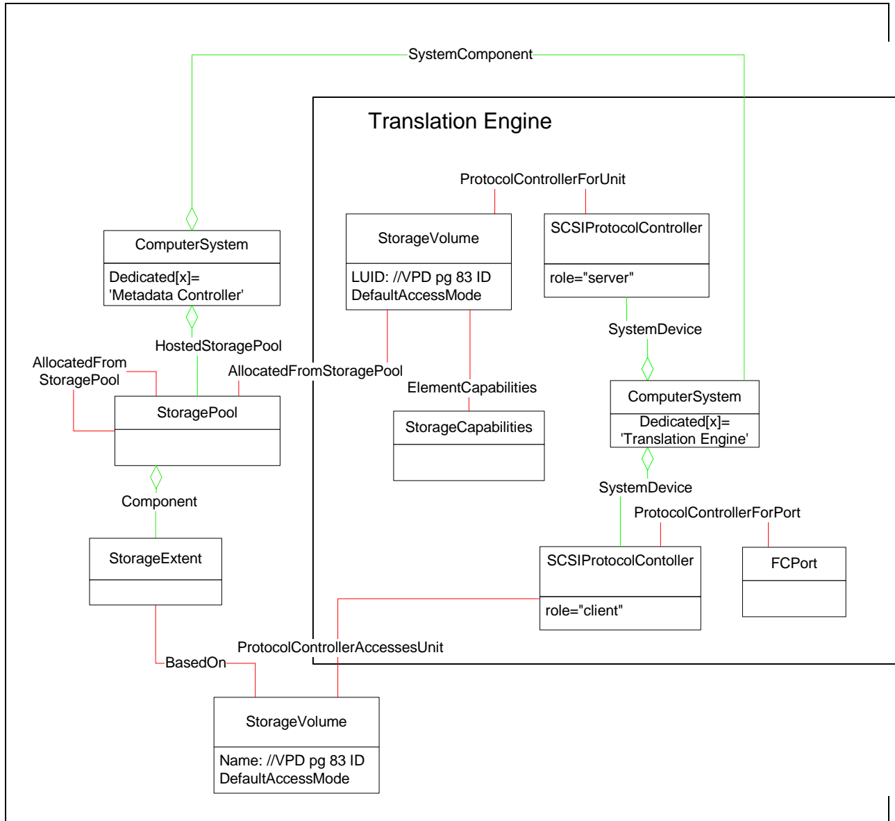
Figure B.13 - Translation Engine Instance Diagram
