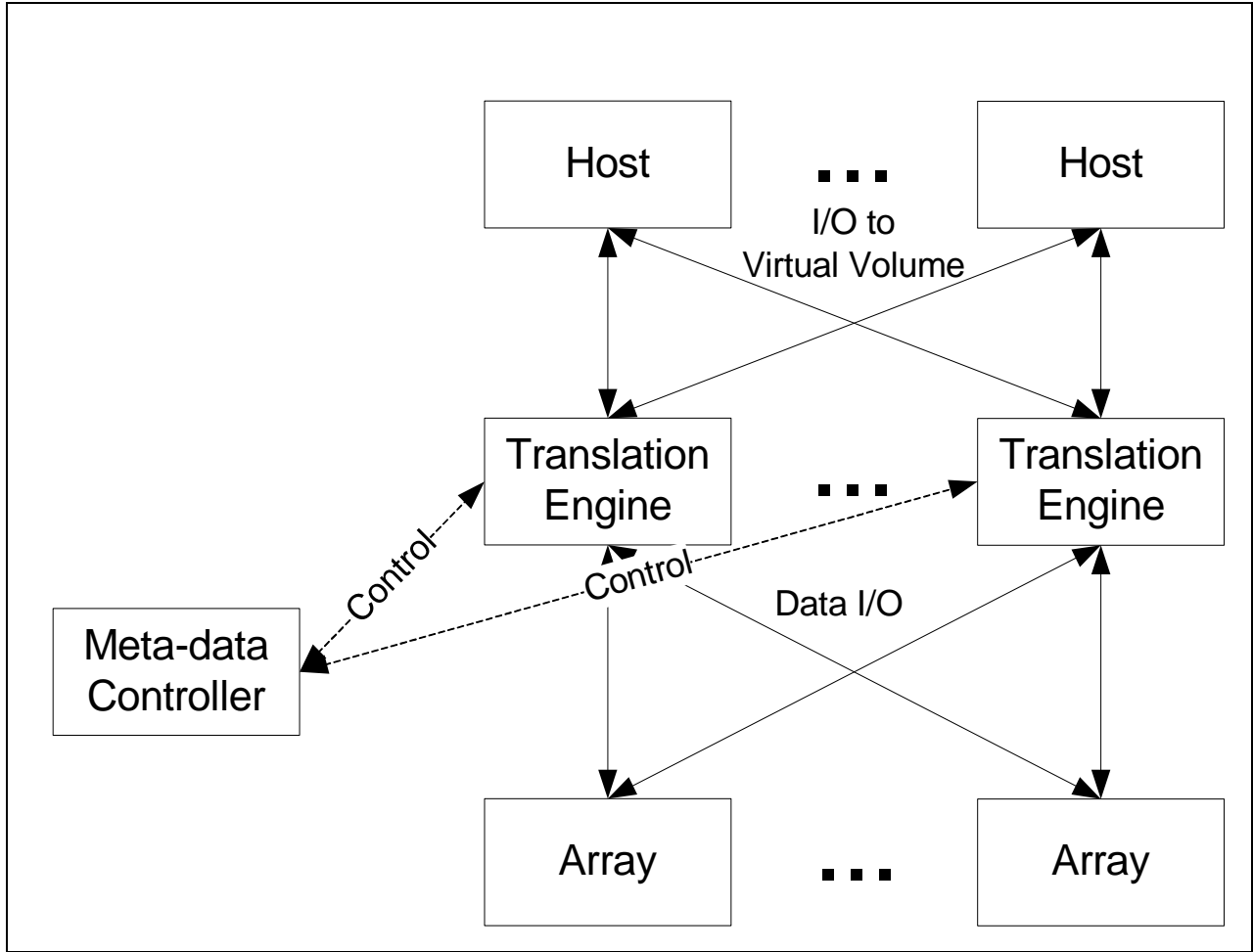
Figure B.10 - Out-of-band Virtualization Block Diagram
