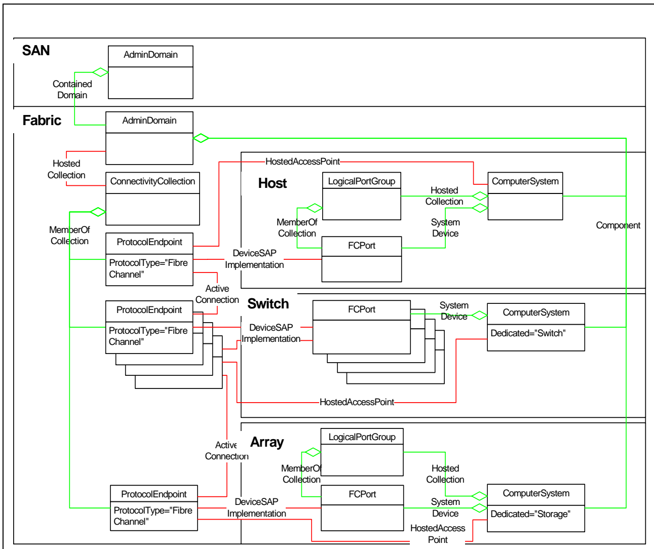
Figure 52 - Fabric Instance Diagram
