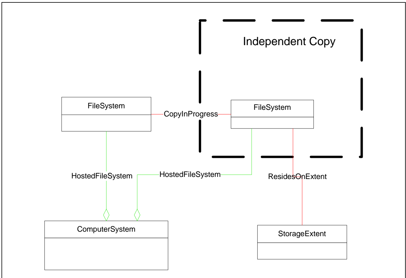
Figure 15 - Filesystem Independent Copy
