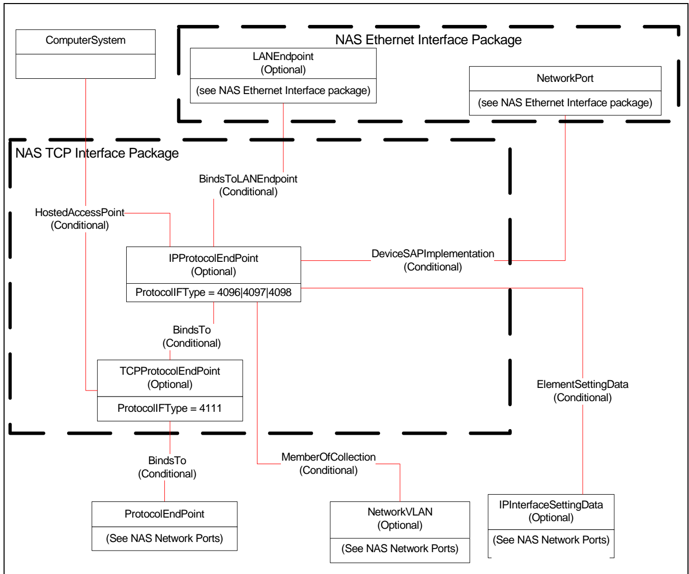
Figure 28 - Optional NAS TCP Interface Modeling
