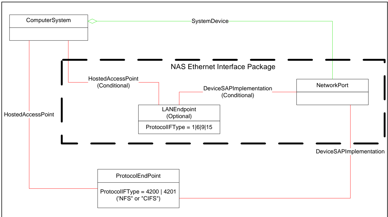
Figure 29 - Mandatory NAS Ethernet Port Modeling
