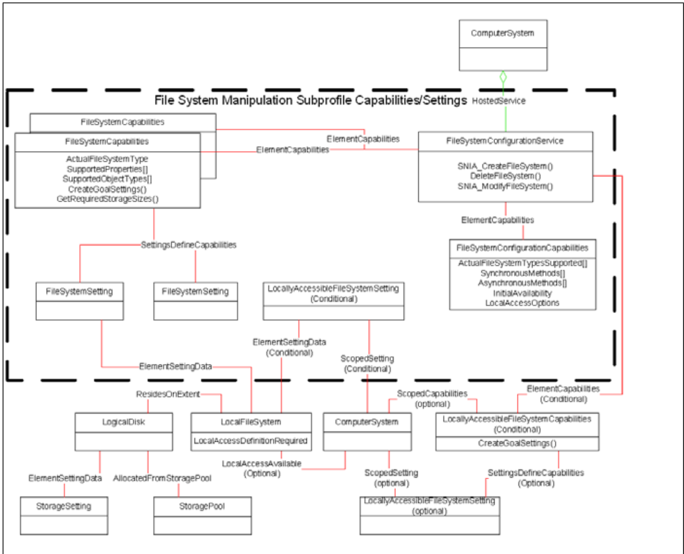
Figure 14 - Capabilities and Settings for Filesystem Creation
