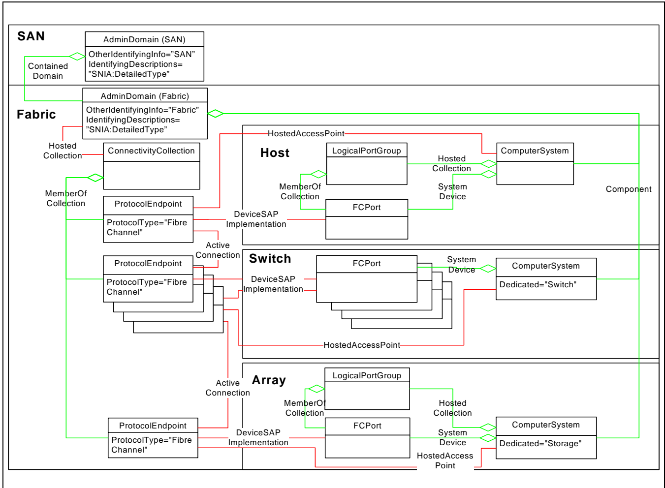
Figure 5 - Fabric Instance
