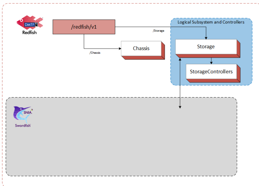
Figure 2: Logical subsystem in swordfish standalone configuration
