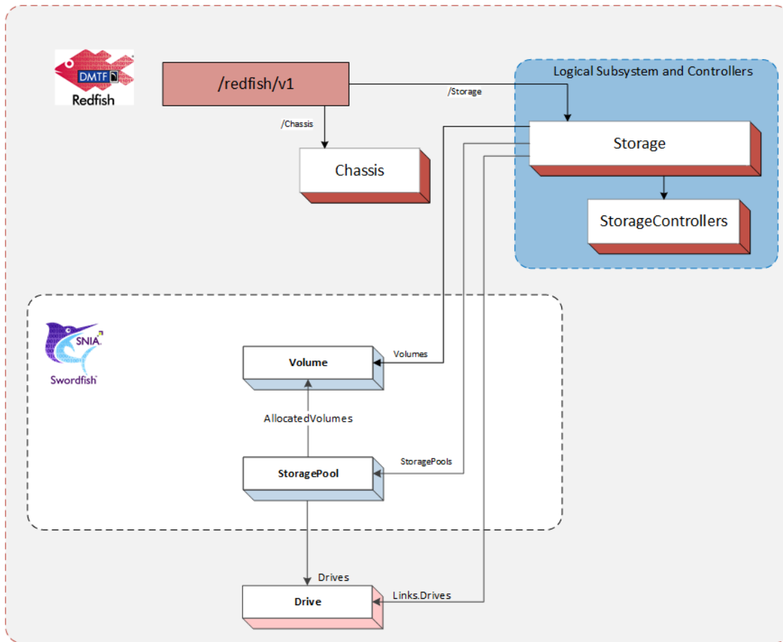
Figure 3: Swordfish Standalone Configuration Example
