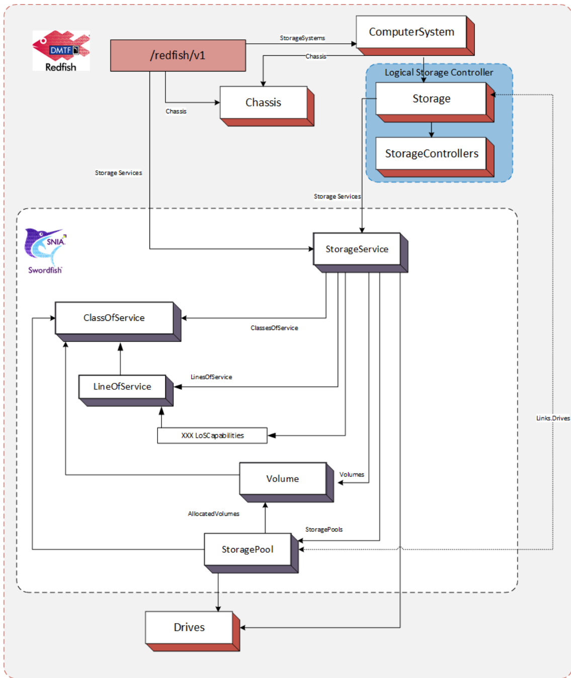
Figure 7: Integrated Service Configuration Example
