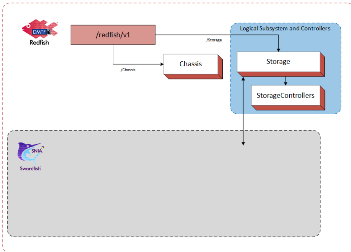
Figure 2: Logical Subsystem in Swordfish Standalone Configuration
